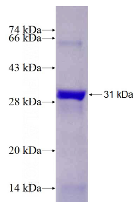
Recombinant Human ANGPTL3 SDS-PAGE
