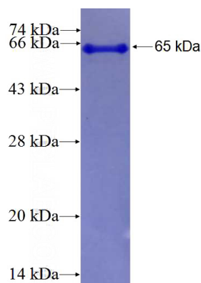
Recombinant Human TIAM2 SDS-PAGE
