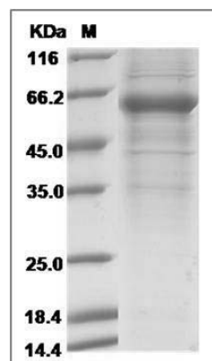
Human B3GALT5 Protein (Fc Tag) SDS-PAGE
