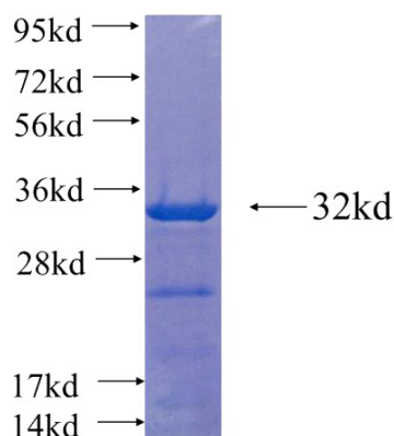
Recombinant Human DNAJC9 SDS-PAGE
