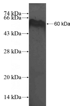
Recombinant Human LRP8 SDS-PAGE
