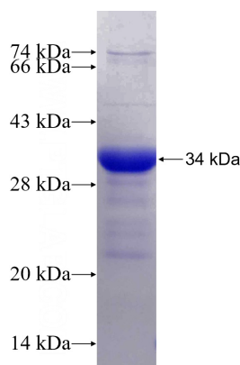
Recombinant Human ZSCAN4 SDS-PAGE
