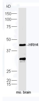
Fig1: Protein: brain(mouse) lysate at 40ug;; Primary: rabbit Anti-HRH4 at 1:300;; Secondary: HRP conjugated Goat-Anti-rabbit IgG(bs-0295G-HRP) at 1: 5000;; Predicted band size: 44 kD; Observed band size: 44 kD
