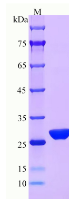
Recombinant Arabidopsis thaliana TGA3 SDS-PAGE
