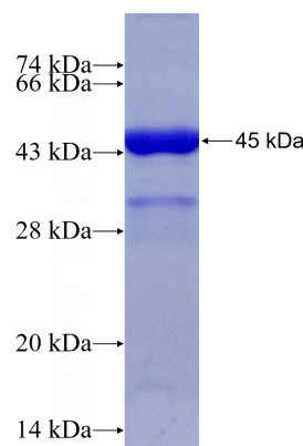
Recombinant Human DSTN SDS-PAGE
