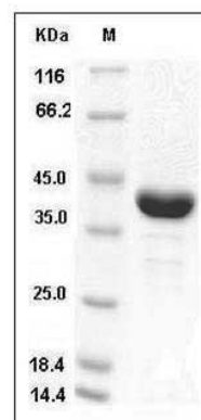
Human AKR1A1 Protein (His Tag) SDS-PAGE
