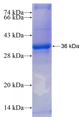
Recombinant Human AHCY SDS-PAGE
