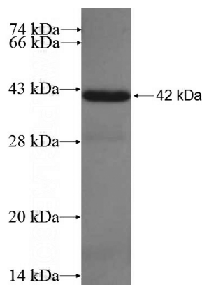
Recombinant Human CRCP SDS-PAGE
