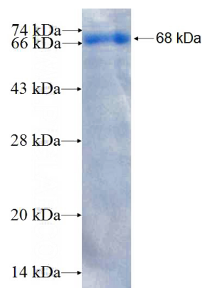
Recombinant Human NSD1 SDS-PAGE
