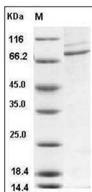
Human CSF1R / MCSF Receptor / CD115 Protein (His & GST Tag) SDS-PAGE
