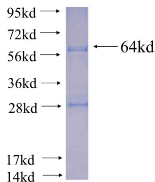
Recombinant human BDH1(Full length) SDS-PAGE
