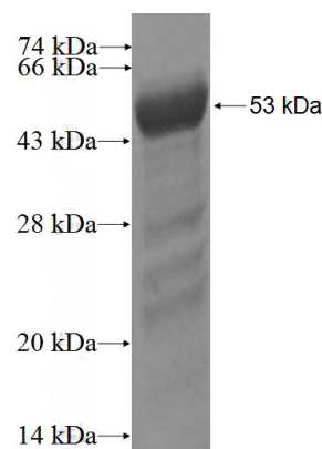
Recombinant Human PPIL4 SDS-PAGE
