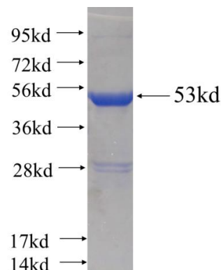
Recombinant human SNX5(Full length) SDS-PAGE
