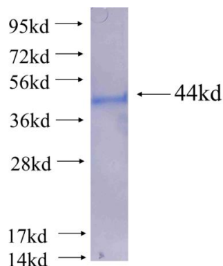
Recombinant human PPIL3(Full length) SDS-PAGE
