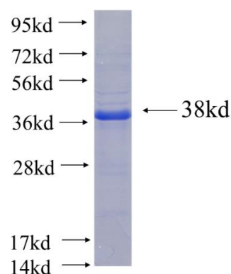
Recombinant human MAP3K7 SDS-PAGE
