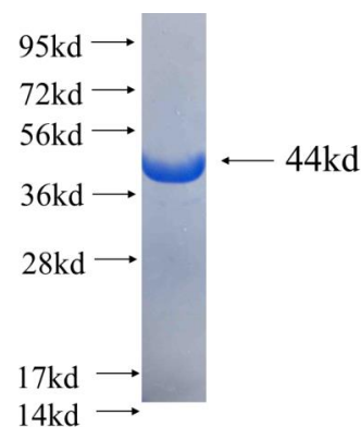
Recombinant Arabidopsis thaliana ACS7 SDS-PAGE
