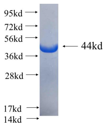
Recombinant Arabidopsis thaliana ACS7 SDS-PAGE
