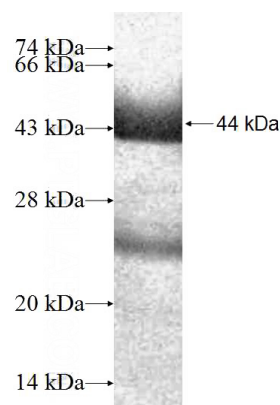
Recombinant Human AGL SDS-PAGE
