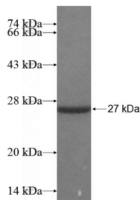
Recombinant Human Occludin SDS-PAGE
