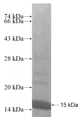
Recombinant Human FSCN2 SDS-PAGE
