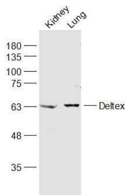
Fig1: Sample:; Kidney (Mouse) Lysate at 40 ug; Lung (Mouse) Lysate at 40 ug; Primary: Anti-Deltex at 1/1000 dilution; Secondary: IRDye800CW Goat Anti-Rabbit IgG at 1/20000 dilution; Predicted band size: 67 kD; Observed band size: 67 kD
