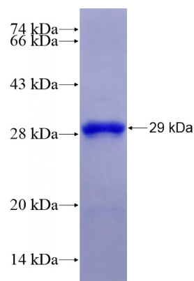
Recombinant Human EEA1 SDS-PAGE
