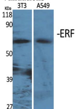
Fig1.; Western Blot analysis of various cells using ERF Polyclonal Antibody cells nucleus extracted by Minute TM Cytoplasmic and Nuclear Fractionation kit (SC-003, Inventbiotech, MN, USA).
