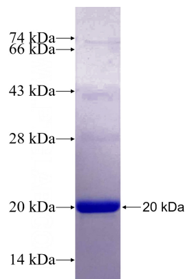
Recombinant Human ACSL3 SDS-PAGE
