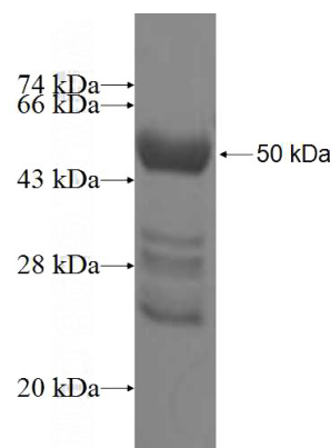
Recombinant Human UNC45A SDS-PAGE
