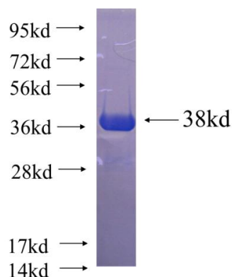
Recombinant human HOXA10 SDS-PAGE
