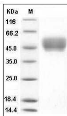
Mouse CD64 / FCGR1 Protein (His Tag) SDS-PAGE
