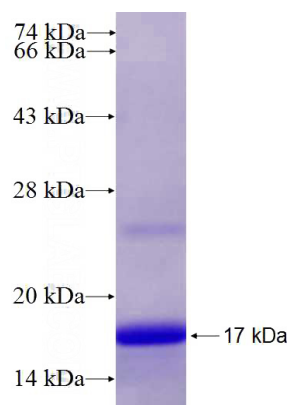
Recombinant Human CTNND2 SDS-PAGE
