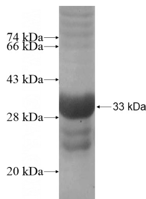
Recombinant Human ZNF493 SDS-PAGE
