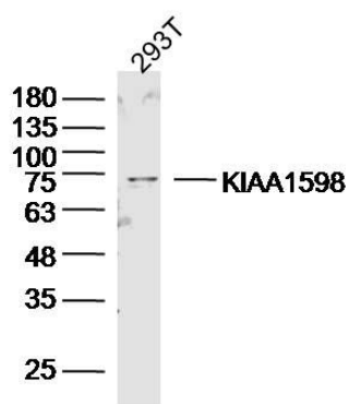
Fig1: Sample:293T Cell (Human) Lysate at 40 ug; Primary: Anti-KIAA1598 at 1/300 dilution; Secondary: IRDye800CW Goat Anti-Rabbit IgG at 1/20000 dilution; Predicted band size: 72kD; Observed band size: 72kD
