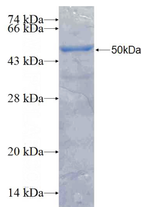
Recombinant Human NLRP10 SDS-PAGE
