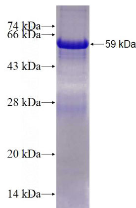
Recombinant Human UBA6 SDS-PAGE
