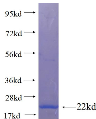
Recombinant human C14orf119 SDS-PAGE
