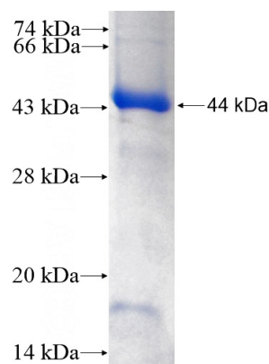
Recombinant Human CXorf22 SDS-PAGE
