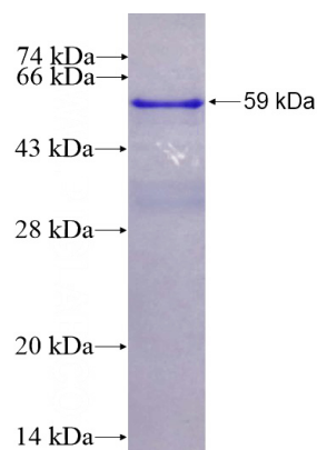
Recombinant Human SMAD4 SDS-PAGE
