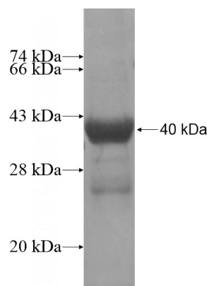
Recombinant Human GPRC5D SDS-PAGE
