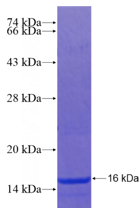
Recombinant Human PRR16 SDS-PAGE
