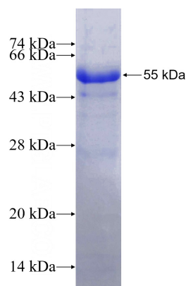
Recombinant Human GABRA3 SDS-PAGE
