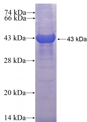
Recombinant Human BMP3 SDS-PAGE
