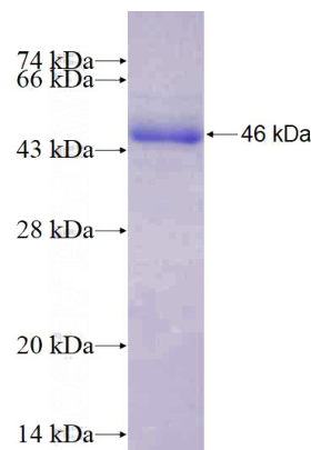
Recombinant Human HDAC5 SDS-PAGE
