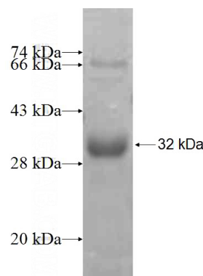
Recombinant Human TMEM98 SDS-PAGE
