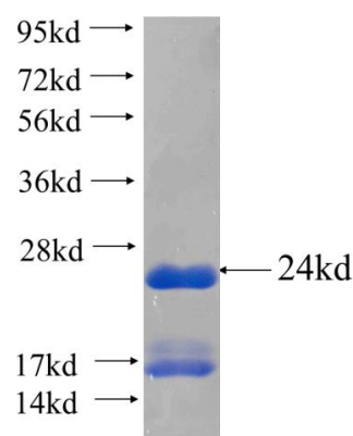
Recombinant human MBP(Full length) SDS-PAGE
