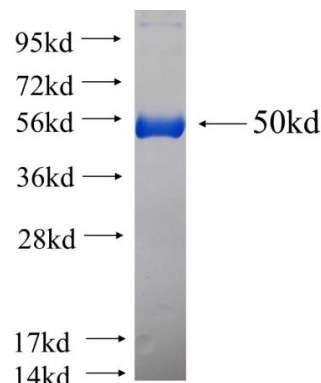
Recombinant human OVCA2(Full length) SDS-PAGE
