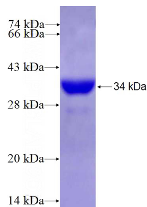
Recombinant Human FAM109B SDS-PAGE
