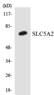
Fig1.; Western blot analysis of the lysates from Jurkat cells using SLC5A2 antibody.
