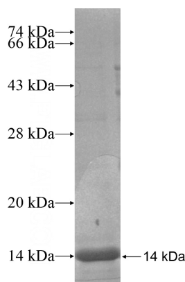
Recombinant Human BSAP,PAX5 SDS-PAGE
