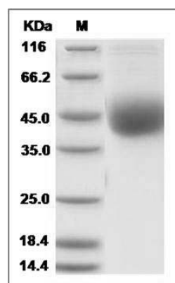
Cynomolgus ART4 Protein (His Tag) SDS-PAGE
